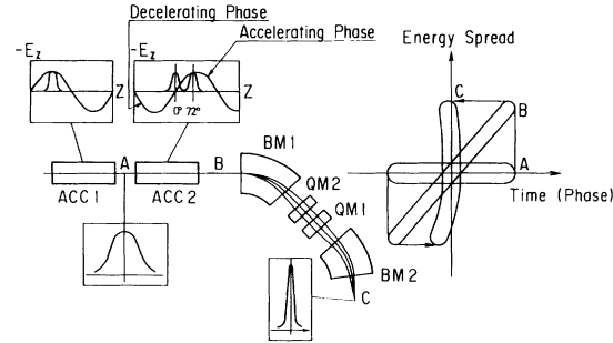
FIG. 2. Schematic drawing of a magnetic pulse compressor and the transformation of a longitudinal phase space distribution. The time or phase stands for the longitudinal coordinate so that the early electrons lie in the right region. The bunches riding on the 0^\circ and 72^\circ rf phases in ACC2 represent the cases of the linear and nonlinear energy modulations.
