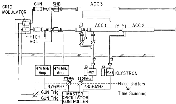
FIG. 1. S-band electron twin linear accelerator of the University of Tokyo.
